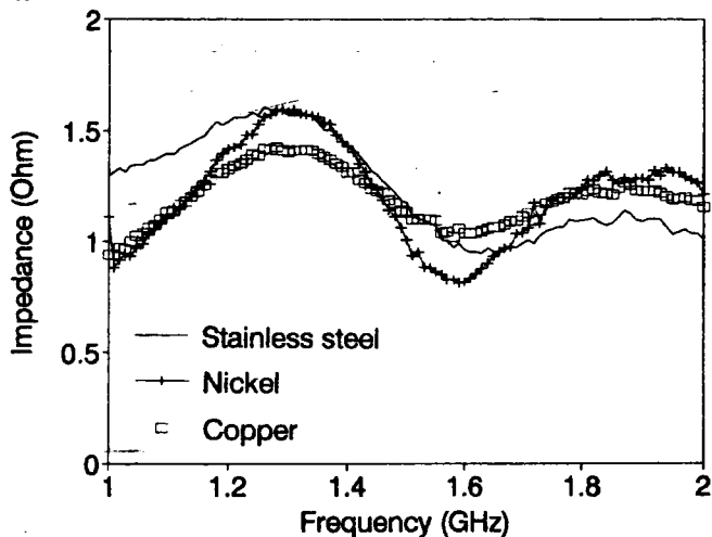
Fig. 6. Variation of surface impedance with frequency of solid copper (□), nickel (+) and stainless steel (—).
