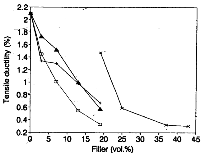
Fig. 9. Variation of tensile ductility with filler volume fraction. +: carbon filaments; □: nickel filaments; ▲: 2 μm diameter Ni fibers; x: 20 μm diameter Ni fibers.
