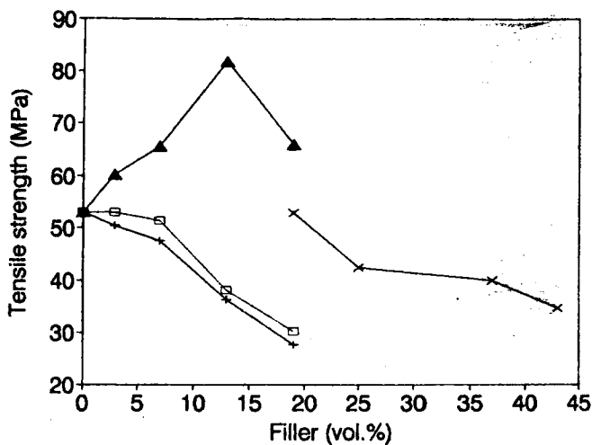
Fig. 7. Variation of tensile strength with filler volume fraction. +: carbon filaments; □: nickel filaments; ▲: 2 μm diameter Ni fibers; x: 20 μm diameter Ni fibers.
